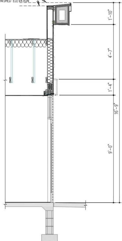
1 WALL SECTION-NEW PARAPET ON TOP OF EXISTING Scale: 3/8"=1'-0"
